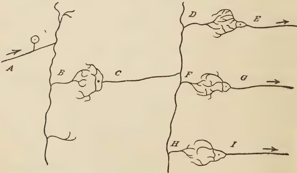
FIG. 2. Multiple response by the branching of a central neurone. (Adapted by permission from Woodworth, Psychology , Holt, New York, 1921, p. 39.)
